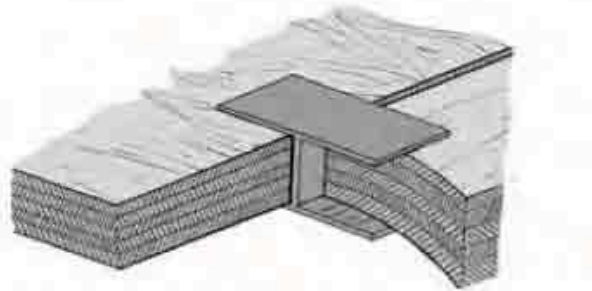
FIGURE 11 - 'H' Clip Detail
