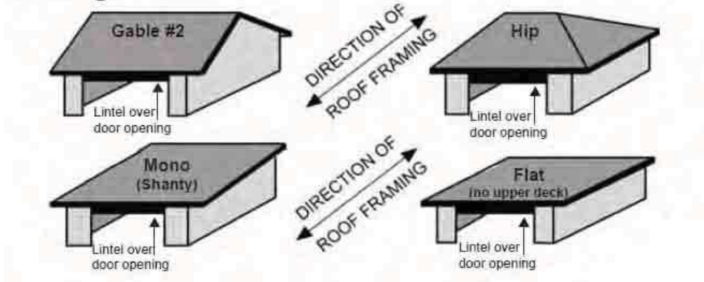
FIGURE 9 - Roof Styles With Lintel SUPPORTING Roof framing.
