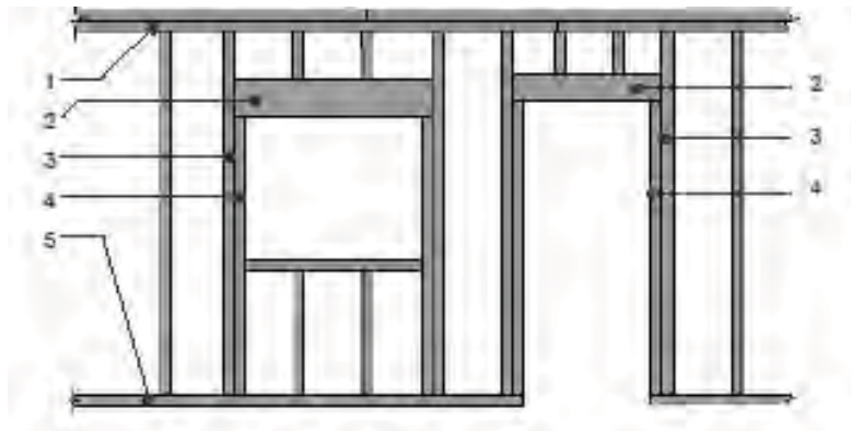
FIGURE 5 – Wall Framing and Lintel Detail
