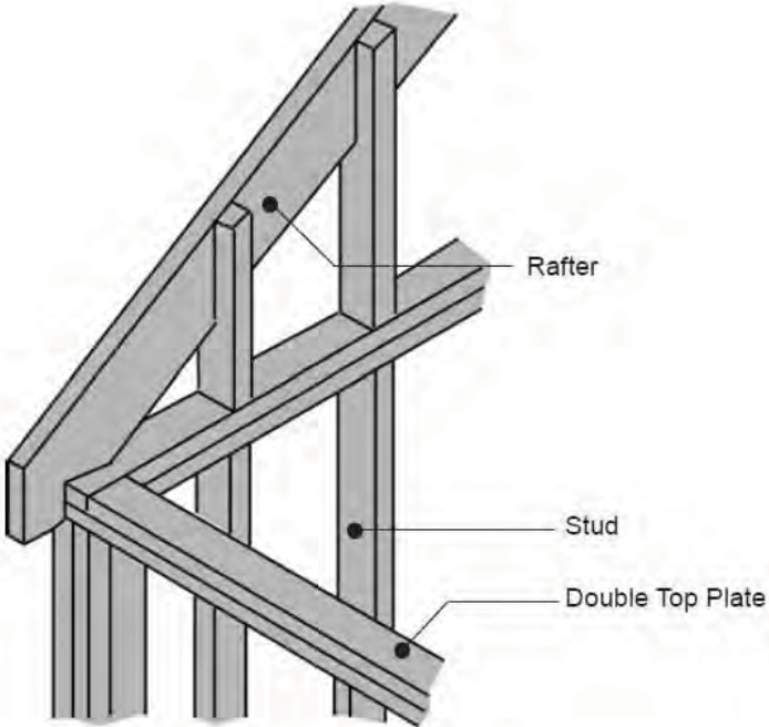
Figure 7 – Exterior Wall Framing at Gable End Detail
